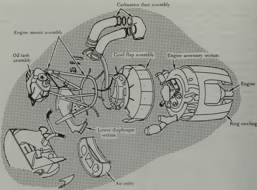
FIGURE 8-1. Exploded view of a typical power package.
